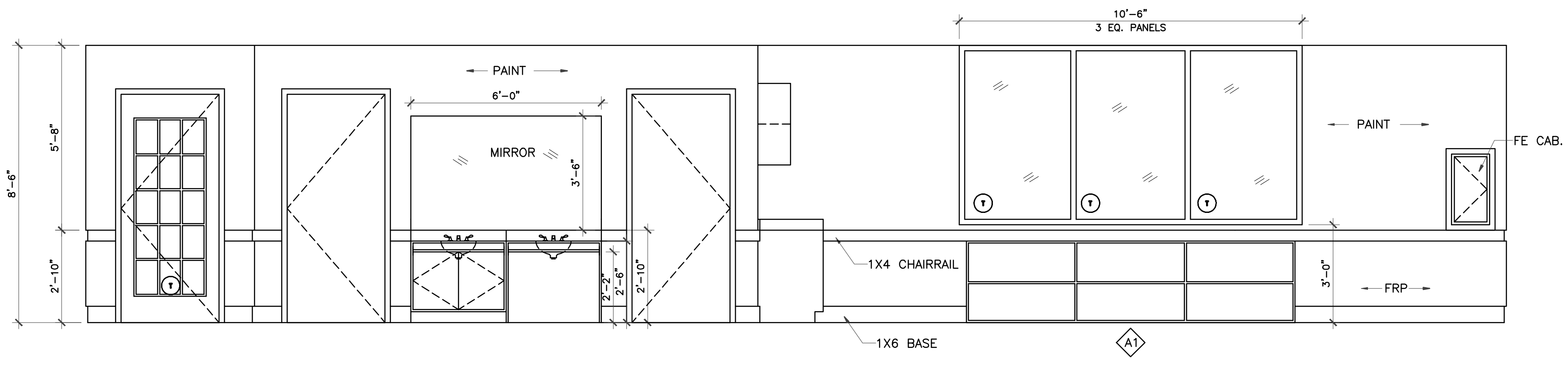
9 CLASSROOM ELEVATION 3/8" = 1'-0"
