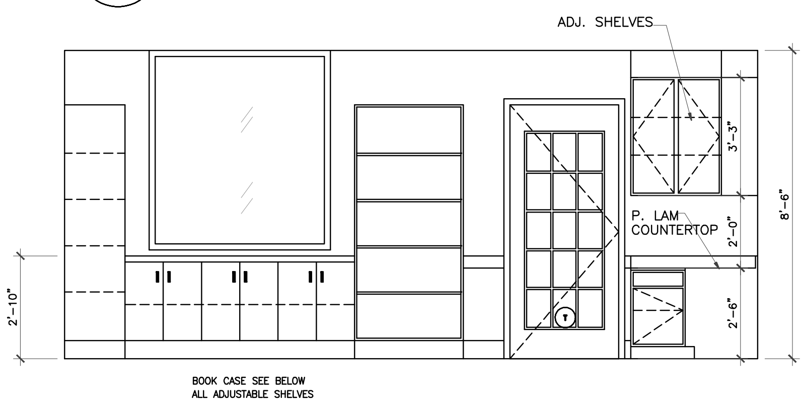
3 LEARNING ELEVATION 3/8" = 1'-0"
