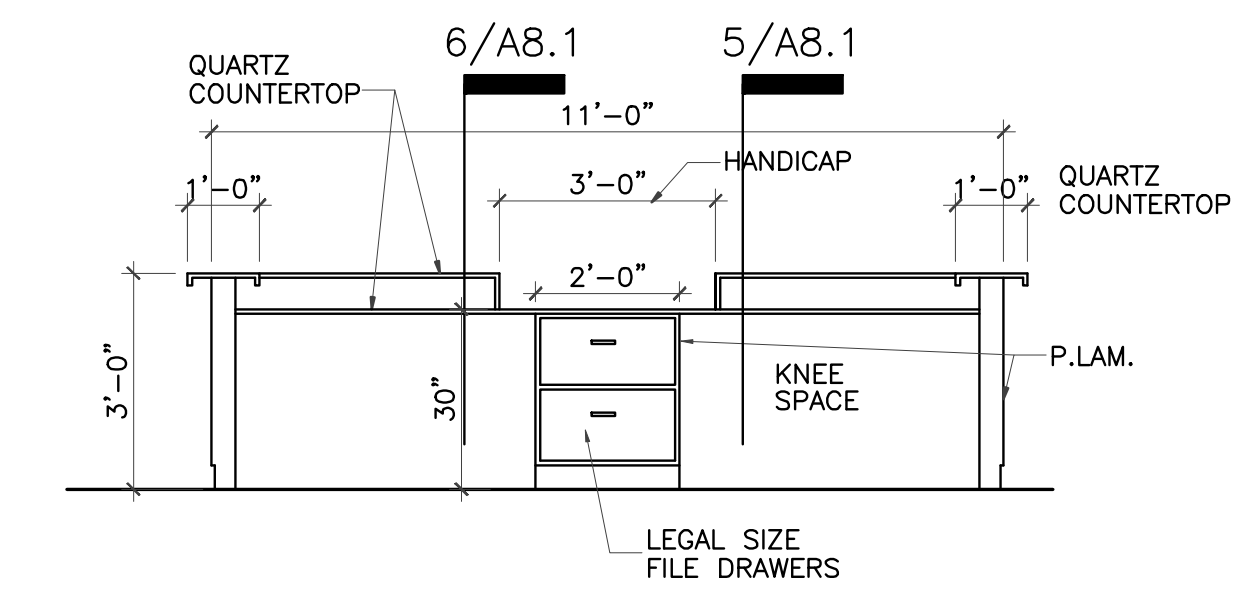
11 MILLWORK ELEVATION-RECEPTION 3/8" = 1'-0"
